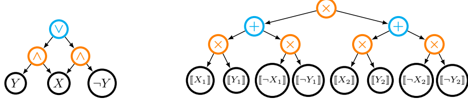
(a) A Boolean circuit that is smooth, decomposable, and deterministic, but not \{X\} -deterministic. (b) A probabilistic circuit that is smooth, decomposable, and \{X_1, X_2\} -deterministic. \llbracket \cdot \rrbracket maps \top to 1 and \perp to 0.
