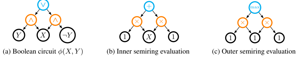
Figure 3: Failure case of 2AMC algorithm on smooth, decomposable, X-first circuit.
